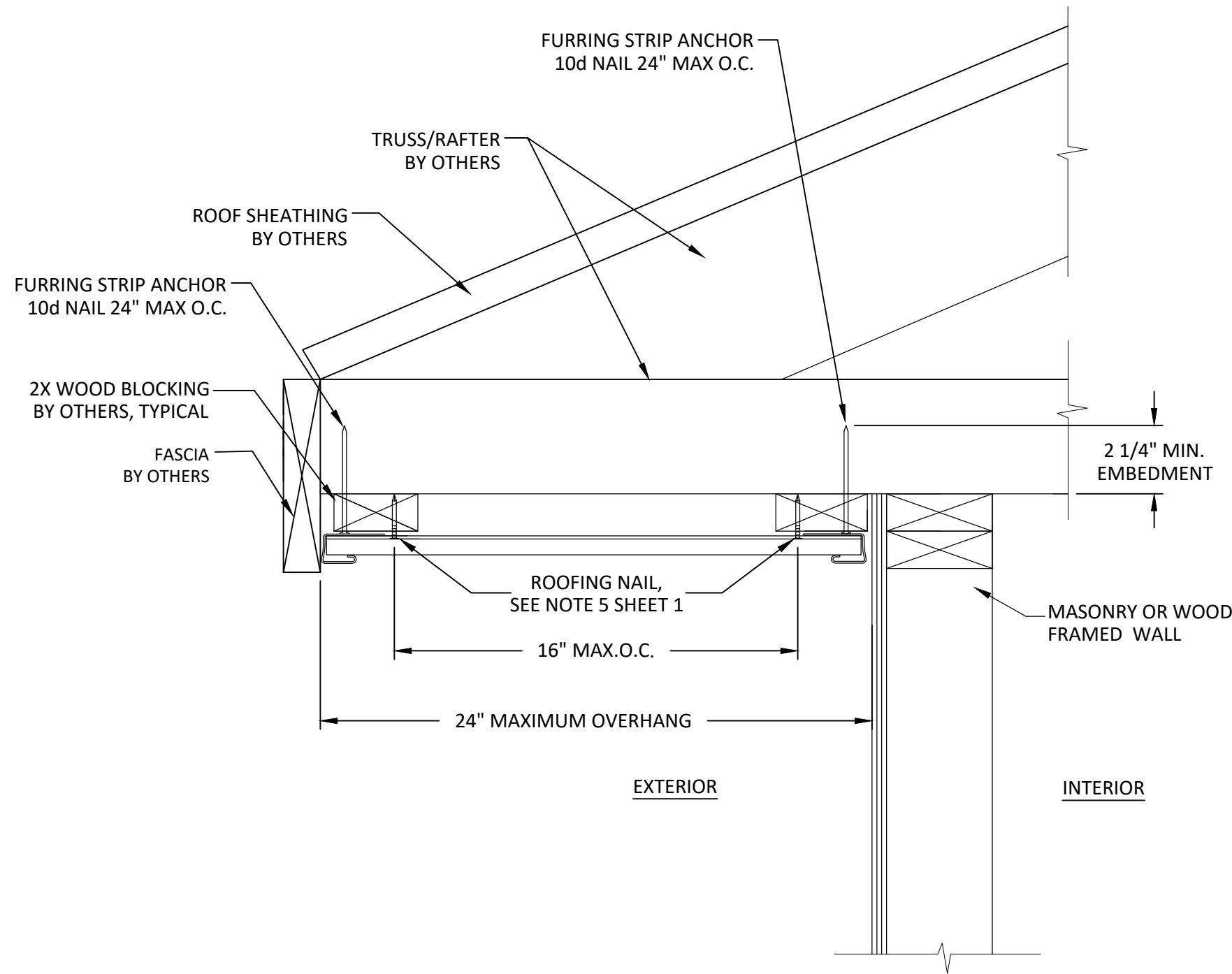
A 2 VERTICAL SECTION SOFFIT INSTALLATION DETAIL 2X WOOD FRAMING OR 1X FURRING STRIP
